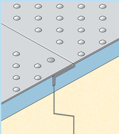
Stainless steel floor, cone pressed
